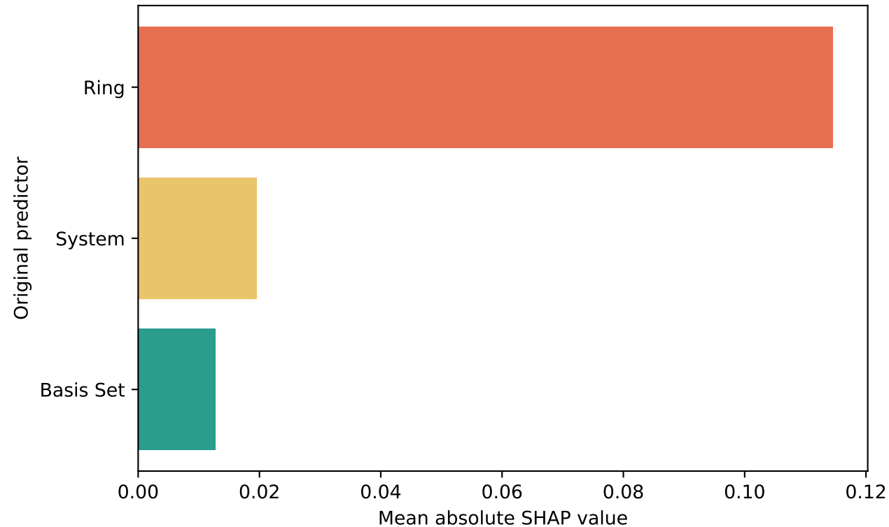
Grouped SHAP importance: norm, |Q_2|_{\text{ring atoms}}
